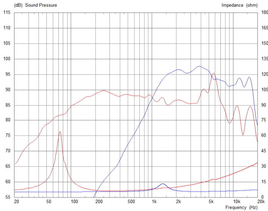
Red: LF response curve | Blue: HF response curve
